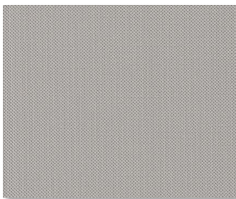
QS22 SHALE
